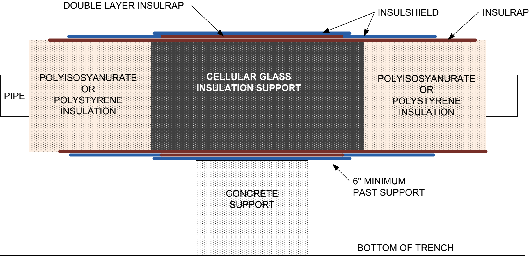
DETAIL SHOWING THE USE OF INSULATION OTHER THAN CELLULAR GLASS ON THE SYSTEM, IF CELLULAR GLASS IS USED ON THE ENTIRE SYSTEM, IGNORE OTHER INSULATIONS SHOWN (DO NOT USE FIBERGLASS)
