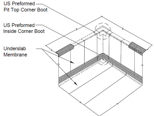
Isometric Overview @ Sump / Elevator Pit
