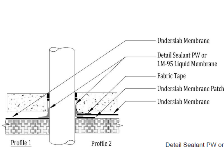
Section @ Underslab Membrane Penetration Detail
