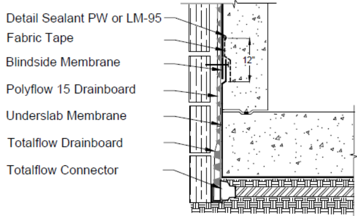
Blindside with Totalflow - Tie in to Underslab
