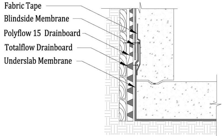
Section @ Blindside Membrane Tie-In to Underslab Membrane
