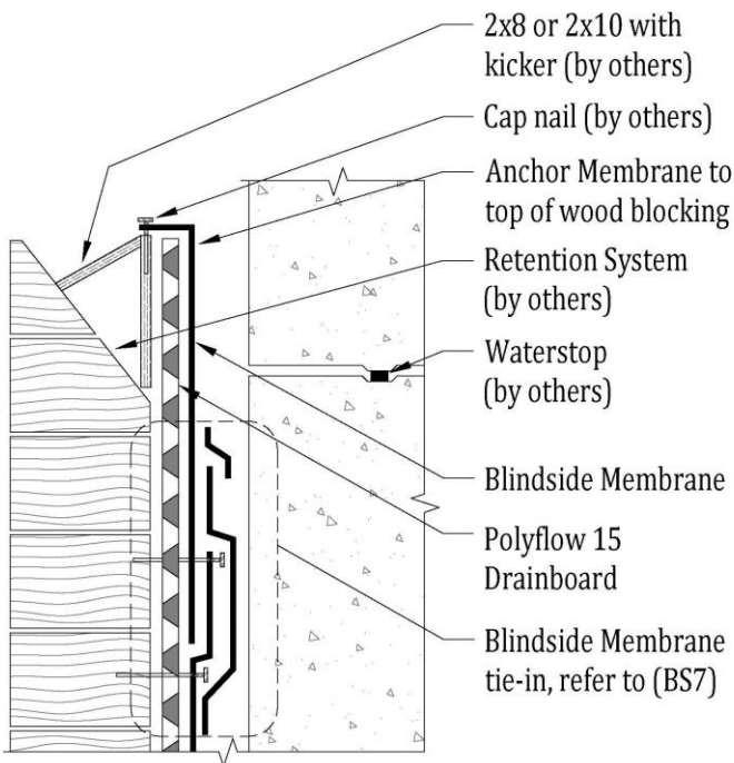
Section @ Blindside Membrane Top of Wall Termination
