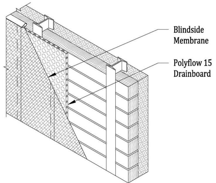
Blindside Membrane with Earth Retention System (Soldier Pile and Lagging shown)
