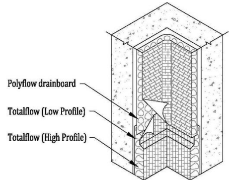
Polyflow Vertical Drainage Board Inside Corner
