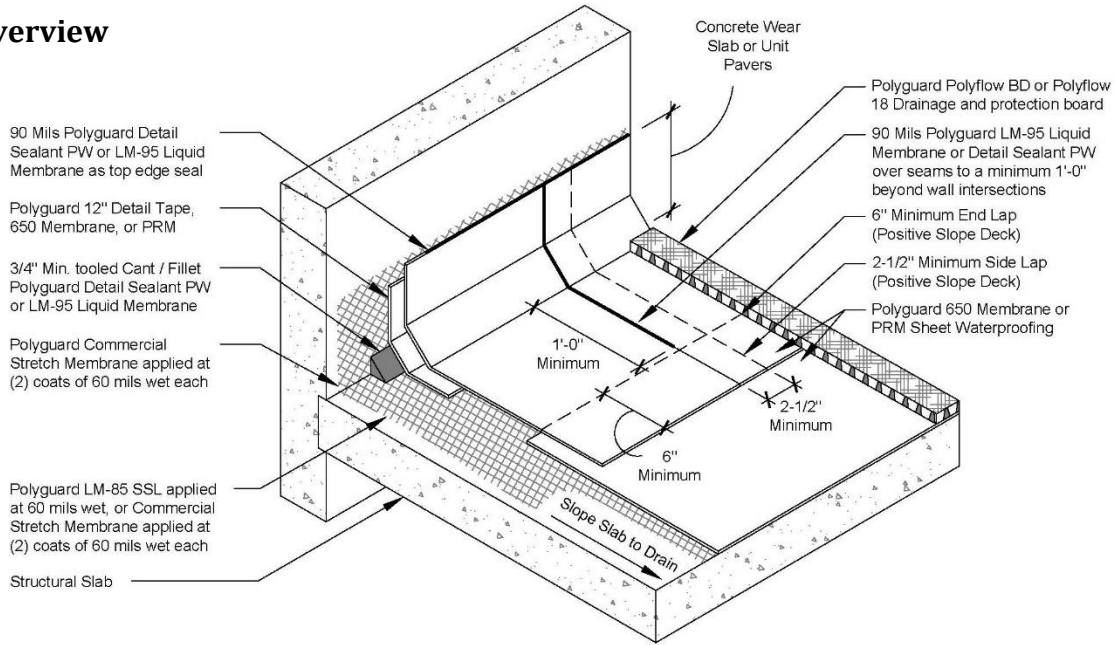
Dual Core Horizontal (DCH) Waterproofing
