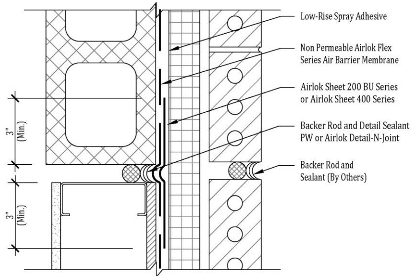
Non Permeable Airlok Flex Series - Substrate Transition
