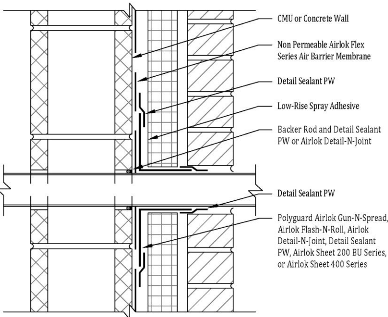
Non Permeable Airlok Flex Series - Wall Penetration
