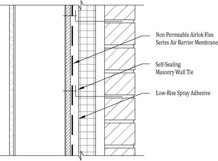
Non Permeable Airlok Flex Series - Typical Wall
