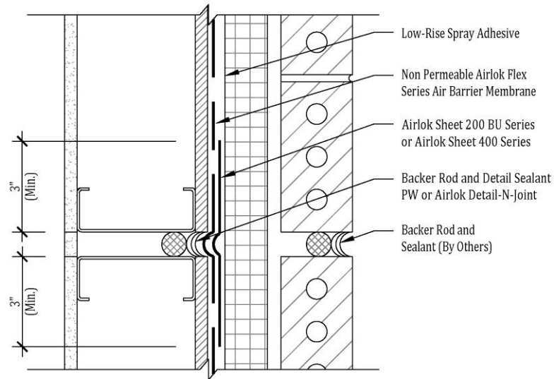
Non Permeable Airlok Flex Series - Expansion Joint
